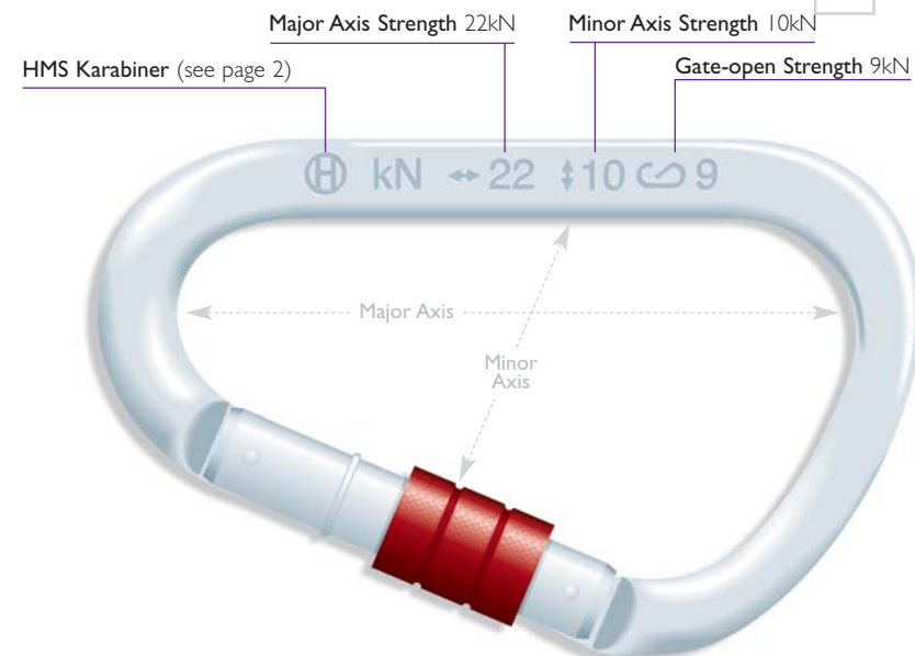
Figure 1.1 Karabiner strength markings
