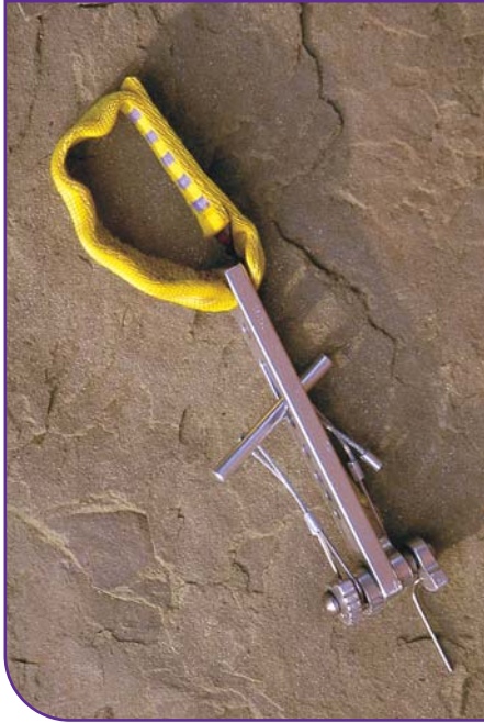
Figure 5.3 Example of a camming unit with a failed trigger wire. It is important to check the trigger wires for broken strands. Manufacturers will repair damaged trigger wires, which helps to avoid the situation shown left.
