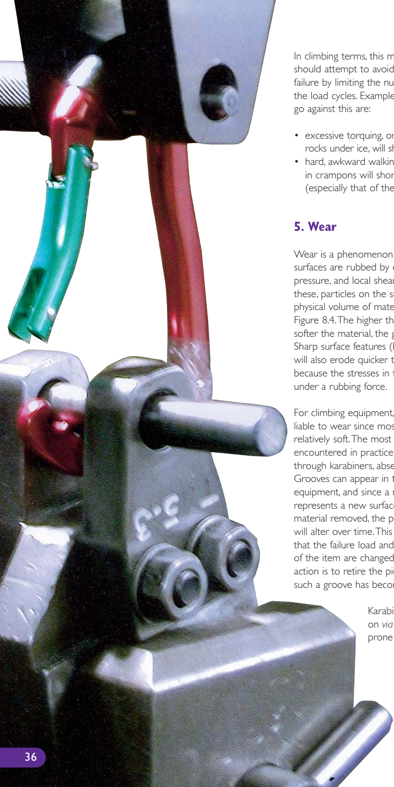
Figure 8.3 Testing the failure load of a karabiner Photo: DMM
