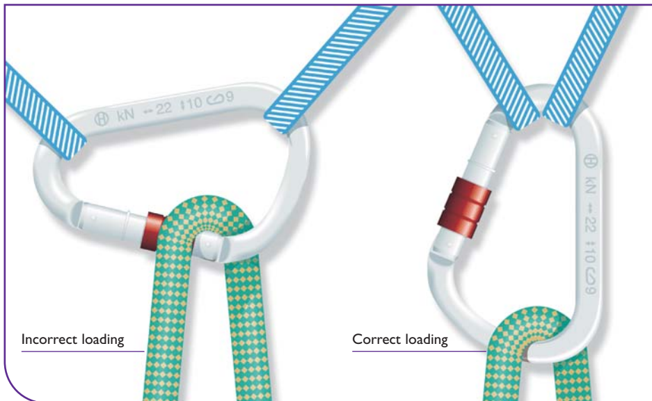
Figure 1.4 Three-way loading of screwgate karabiner
