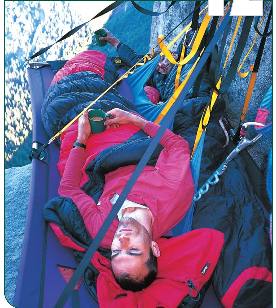
Figure 12.1 Neil Bentley and Richard Heap appreciating slings in Yosemite, USA
