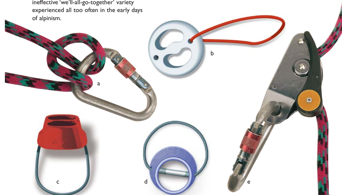
Figure 7.1 Belay and abseil methods and devices a: Italian Hitch, b: Sticht Plate, c: ATC, d: Latok Tuber, e: Grigri
